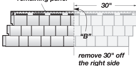
drill 3/16" diameter hole at midpoint of remaining panel
